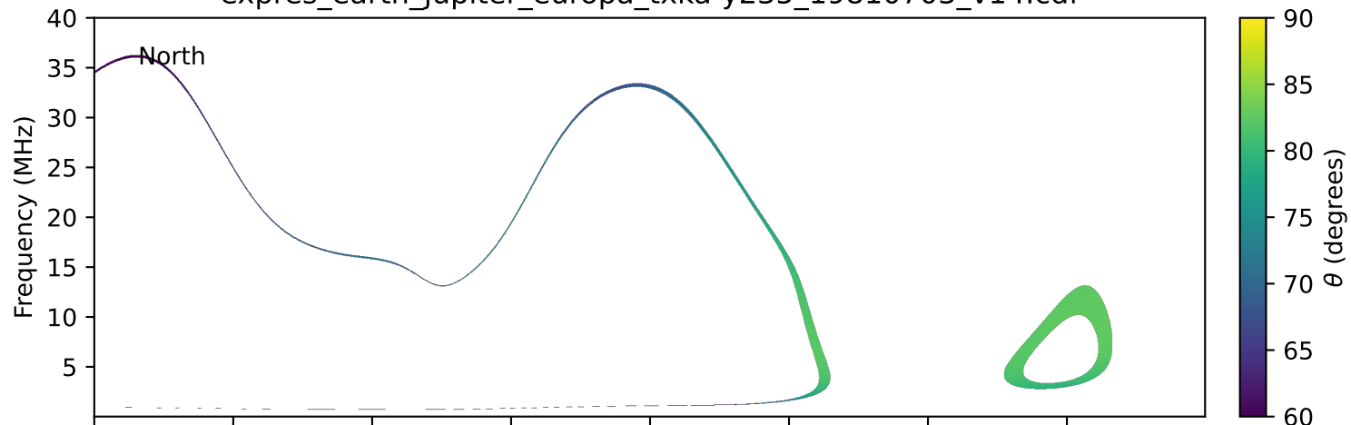
expres_earth_jupiter_europa_txka-y235_19810703_v14.cdf
