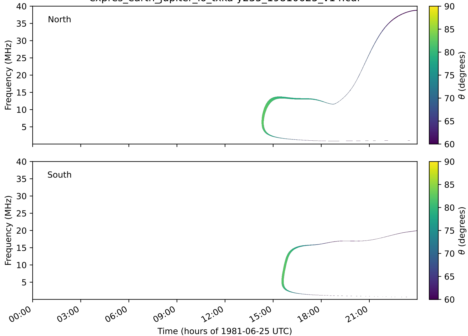
expres_earth_jupiter_io_txka-y235_19810625_v14.cdf
