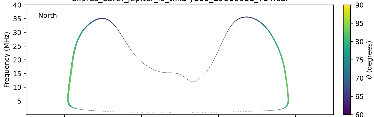
expres_earth_jupiter_io_txka-y235_19810622_v14.cdf
