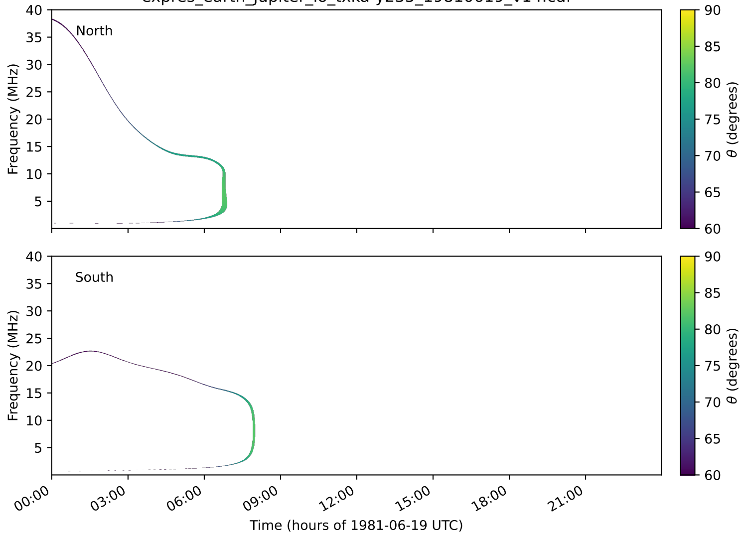
expres_earth_jupiter_io_txka-y235_19810619_v14.cdf
