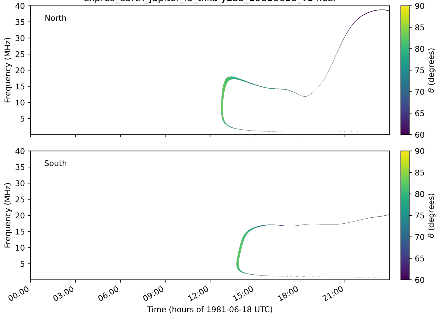
expres_earth_jupiter_io_txka-y235_19810618_v14.cdf
