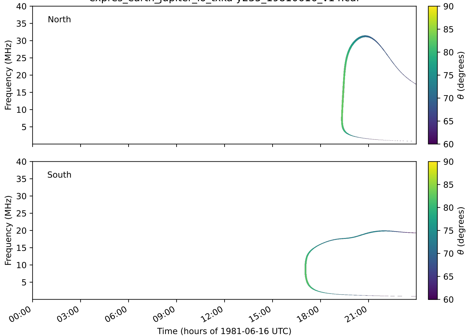
expres_earth_jupiter_io_txka-y235_19810616_v14.cdf
