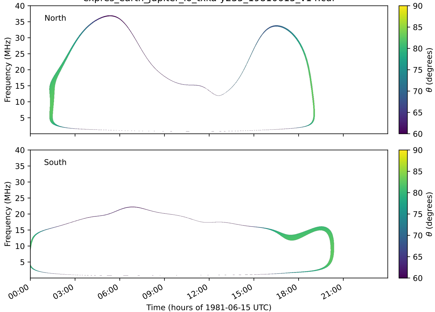
expres_earth_jupiter_io_txka-y235_19810615_v14.cdf
