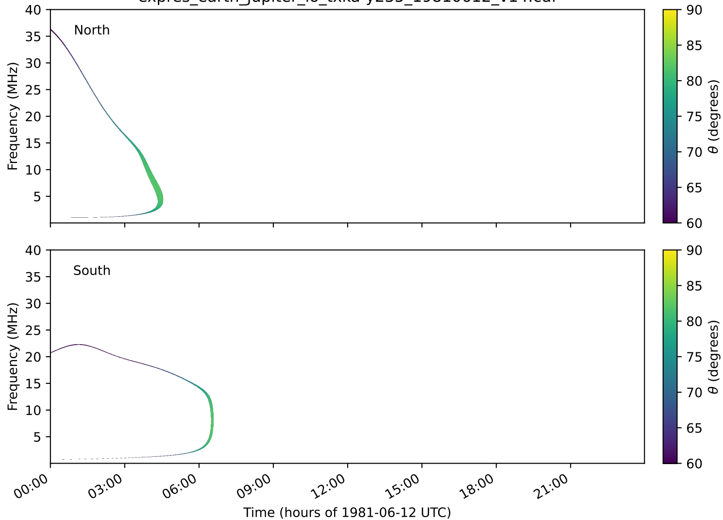
expres_earth_jupiter_io_txka-y235_19810612_v14.cdf
