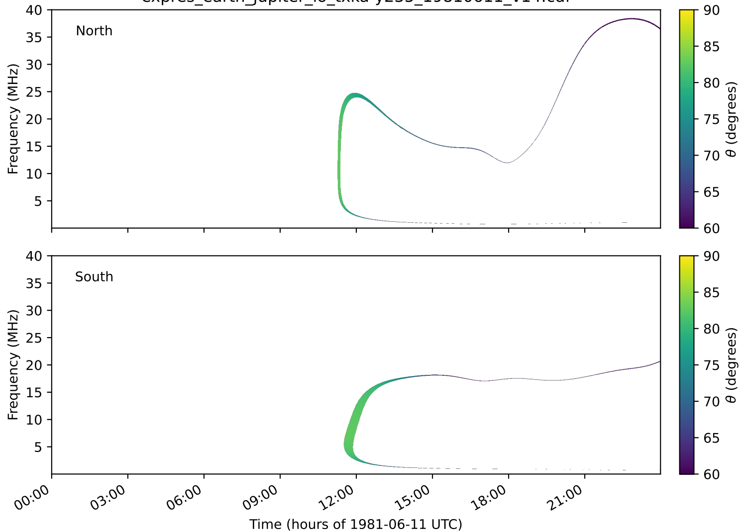
expres_earth_jupiter_io_txka-y235_19810611_v14.cdf
