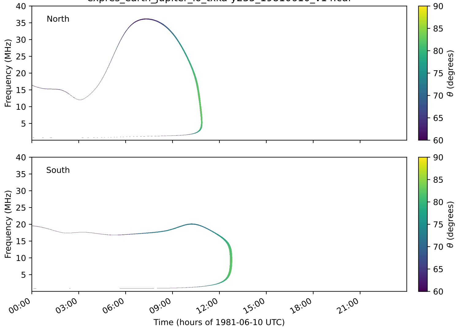
expres_earth_jupiter_io_txka-y235_19810610_v14.cdf
