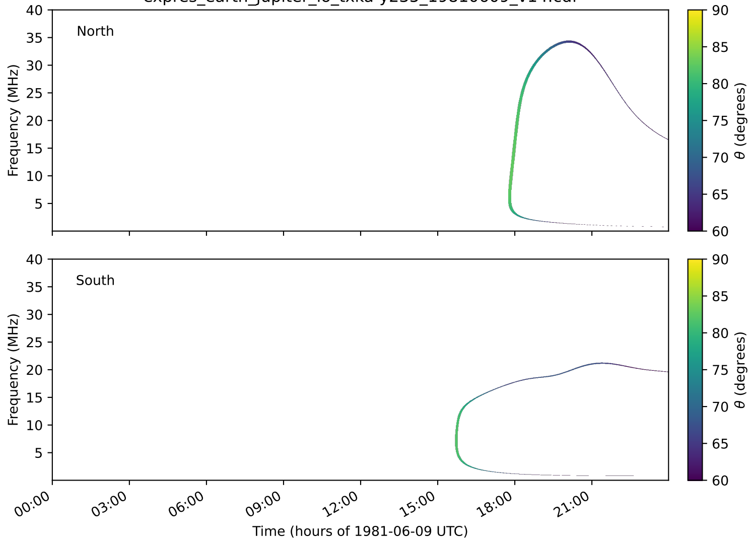
expres_earth_jupiter_io_txka-y235_19810609_v14.cdf
