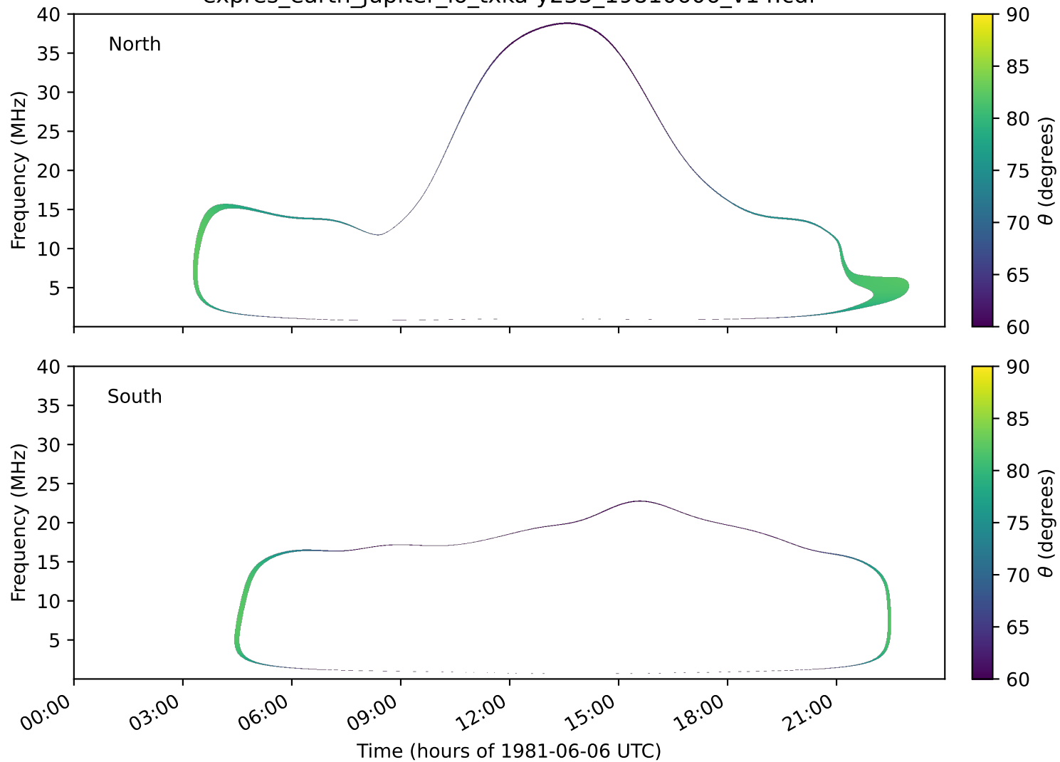
expres_earth_jupiter_io_txka-y235_19810606_v14.cdf
