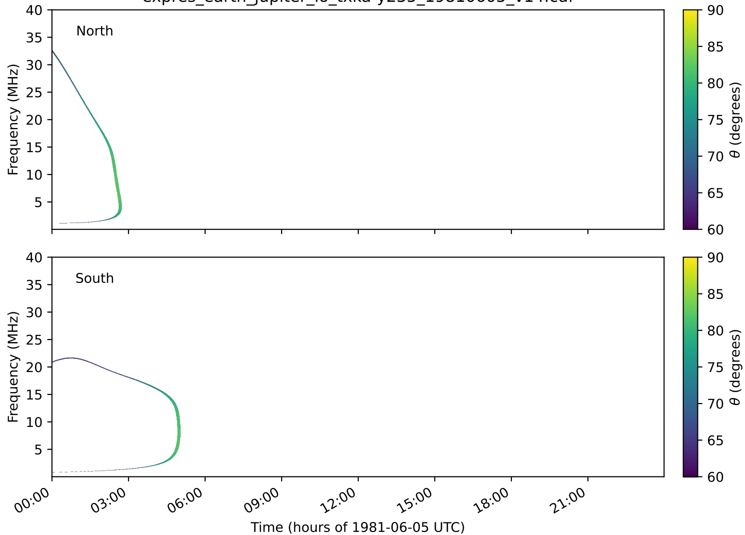
expres_earth_jupiter_io_txka-y235_19810605_v14.cdf
