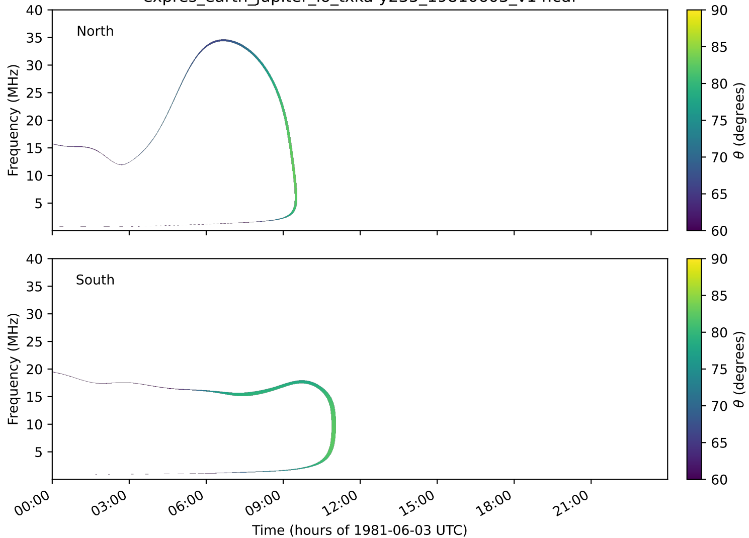
expres_earth_jupiter_io_txka-y235_19810603_v14.cdf
