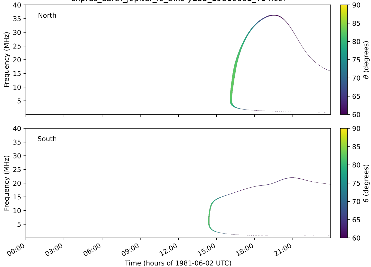
expres_earth_jupiter_io_txka-y235_19810602_v14.cdf
