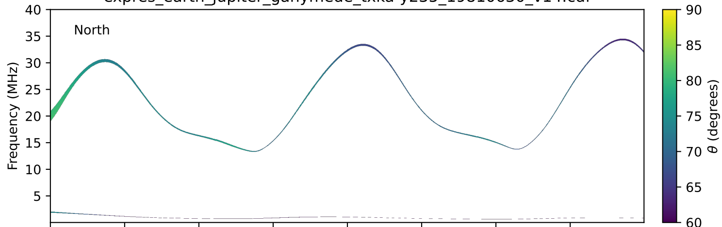
expres_earth_jupiter_ganymede_txka-y235_19810630_v14.cdf
