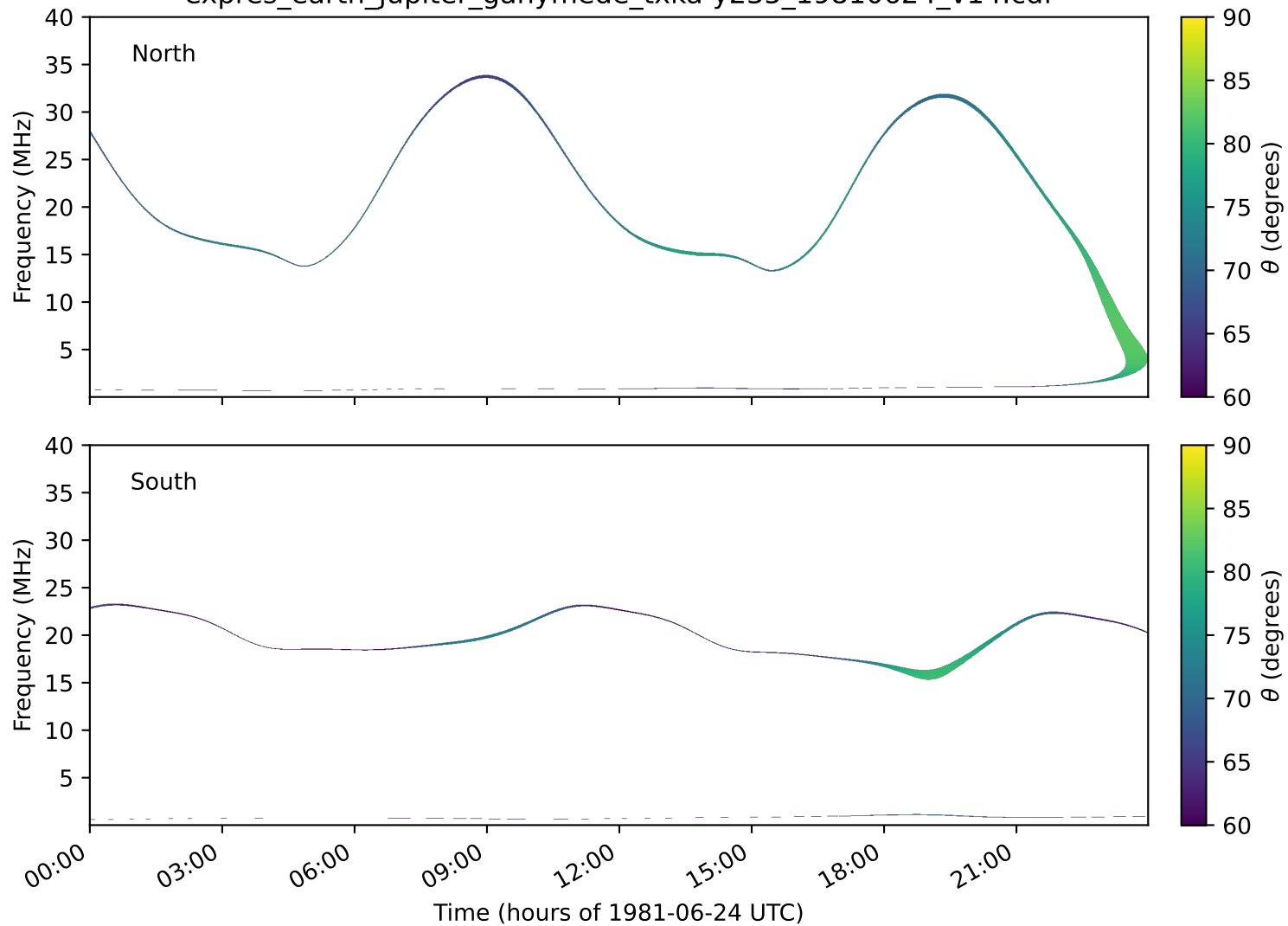
expres_earth_jupiter_ganymede_txka-y235_19810624_v14.cdf
