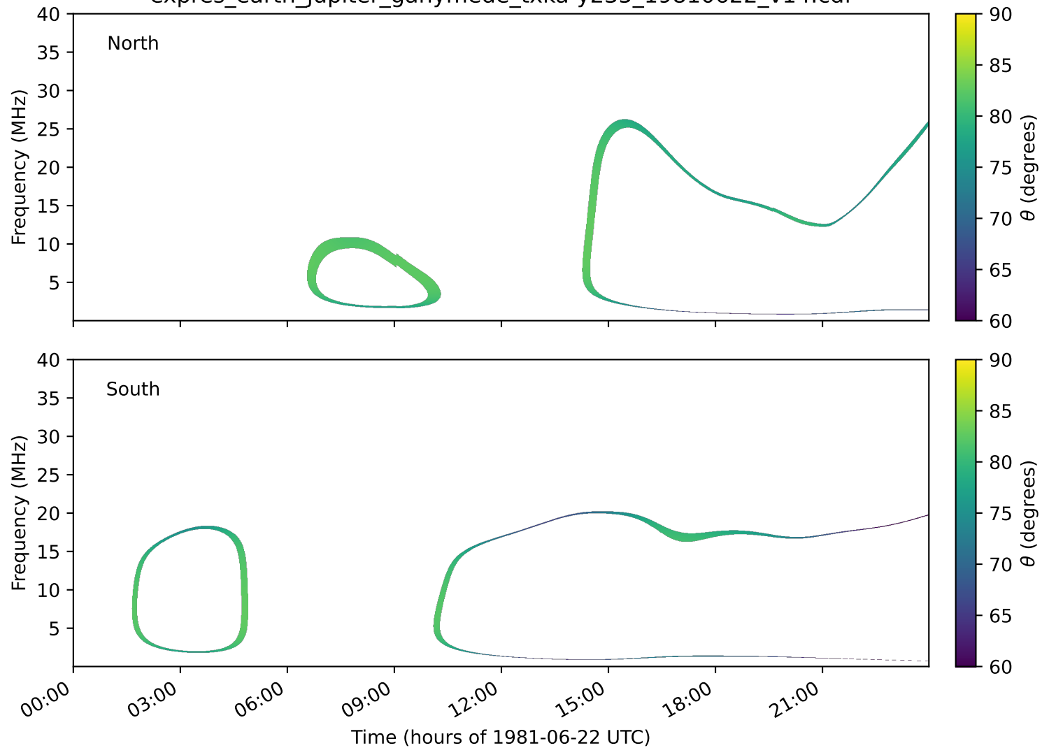
expres_earth_jupiter_ganymede_txka-y235_19810622_v14.cdf
