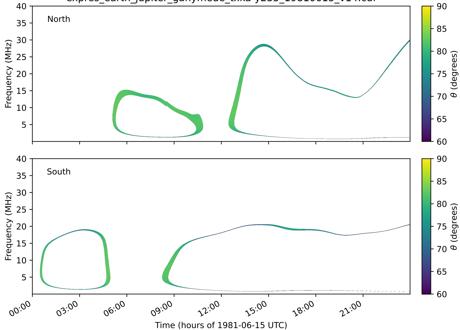
expres_earth_jupiter_ganymede_txka-y235_19810615_v14.cdf
