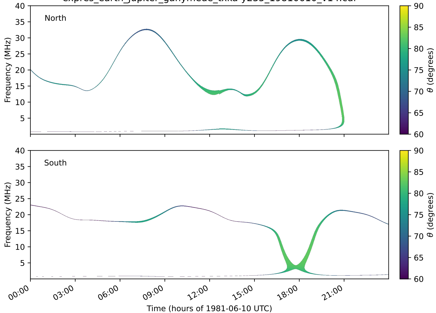
expres_earth_jupiter_ganymede_txka-y235_19810610_v14.cdf
