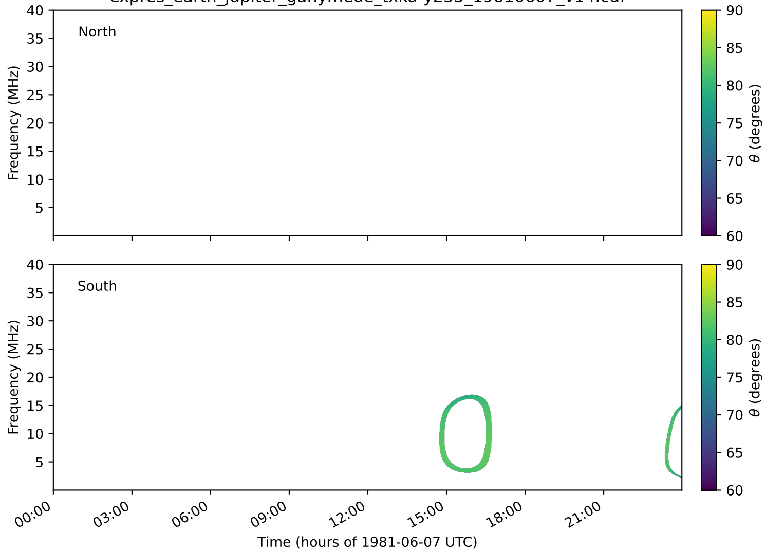
expres_earth_jupiter_ganymede_txka-y235_19810607_v14.cdf
