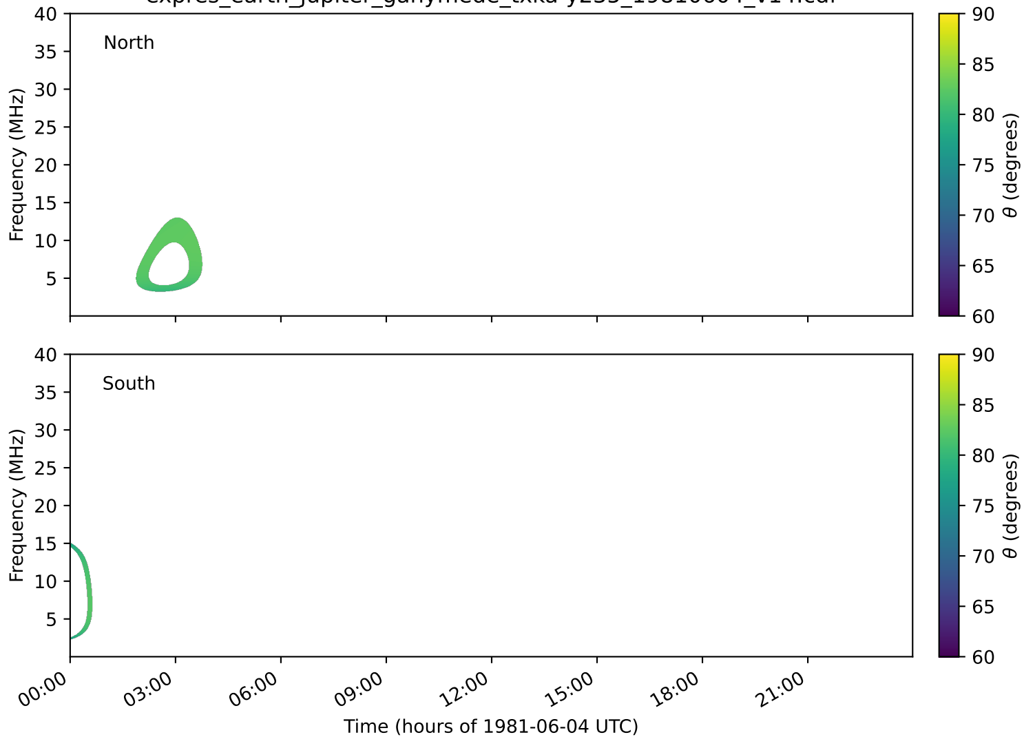
expres_earth_jupiter_ganymede_txka-y235_19810604_v14.cdf
