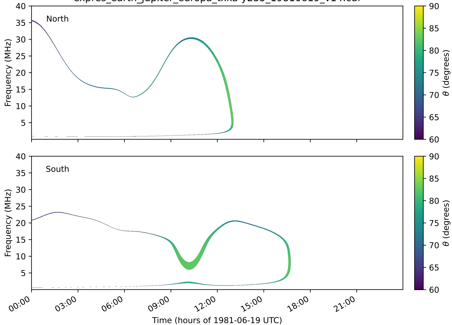
expres_earth_jupiter_europa_txka-y235_19810619_v14.cdf
