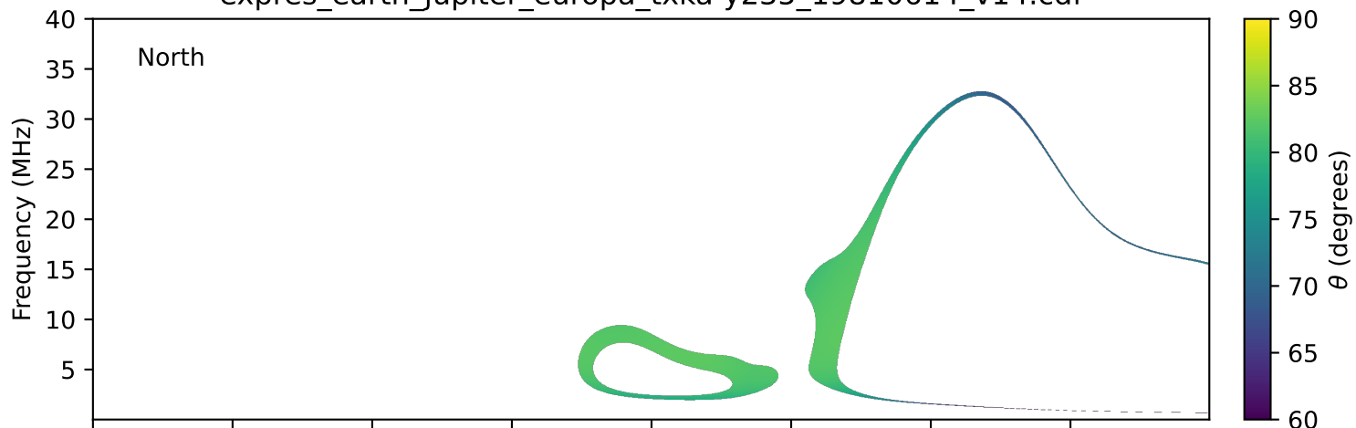
expres_earth_jupiter_europa_txka-y235_19810614_v14.cdf
