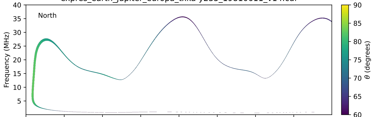
expres_earth_jupiter_europa_txka-y235_19810611_v14.cdf
