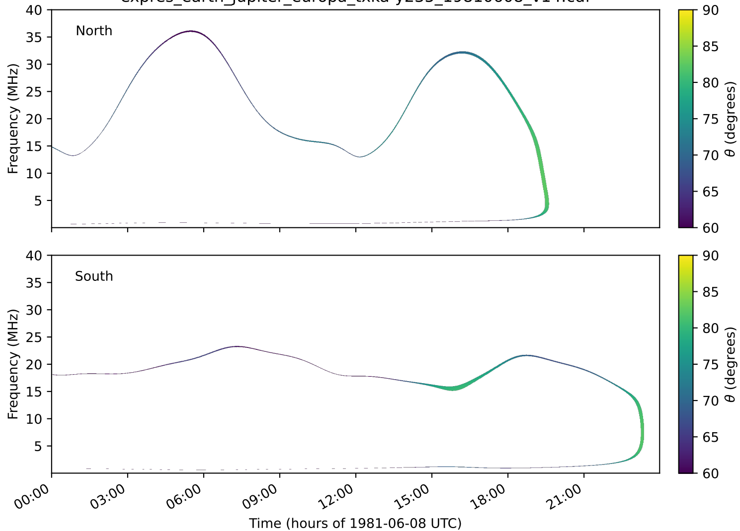
expres_earth_jupiter_europa_txka-y235_19810608_v14.cdf
