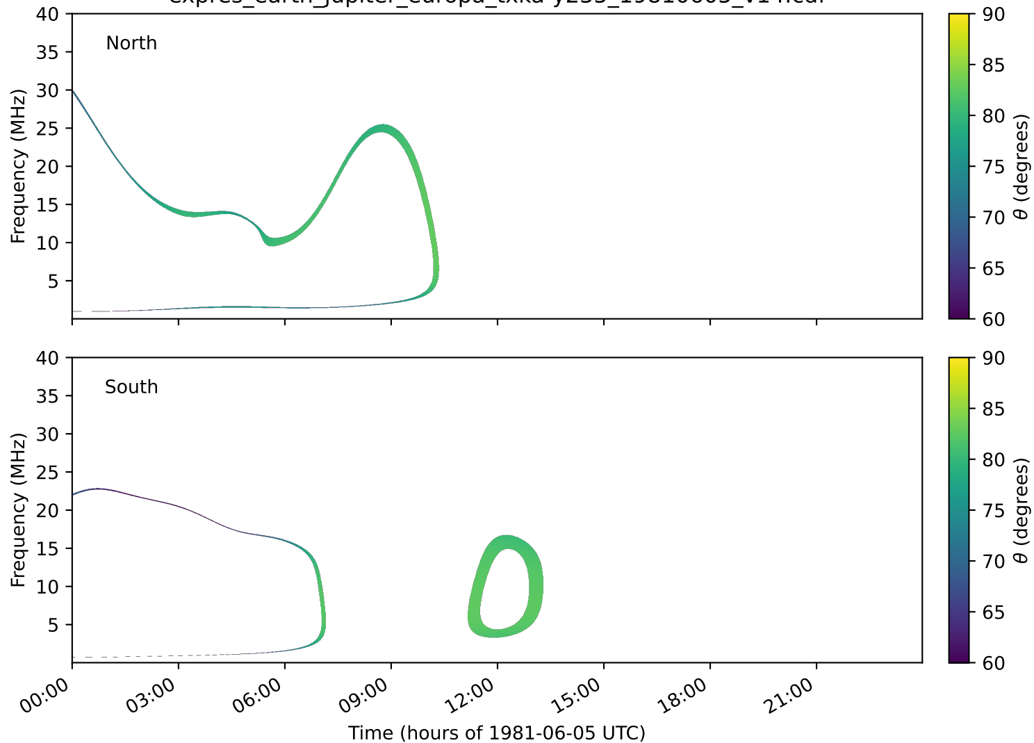
expres_earth_jupiter_europa_txka-y235_19810605_v14.cdf
