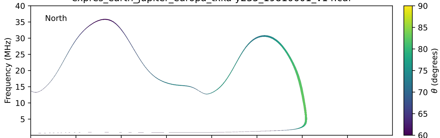
expres_earth_jupiter_europa_txka-y235_19810601_v14.cdf
