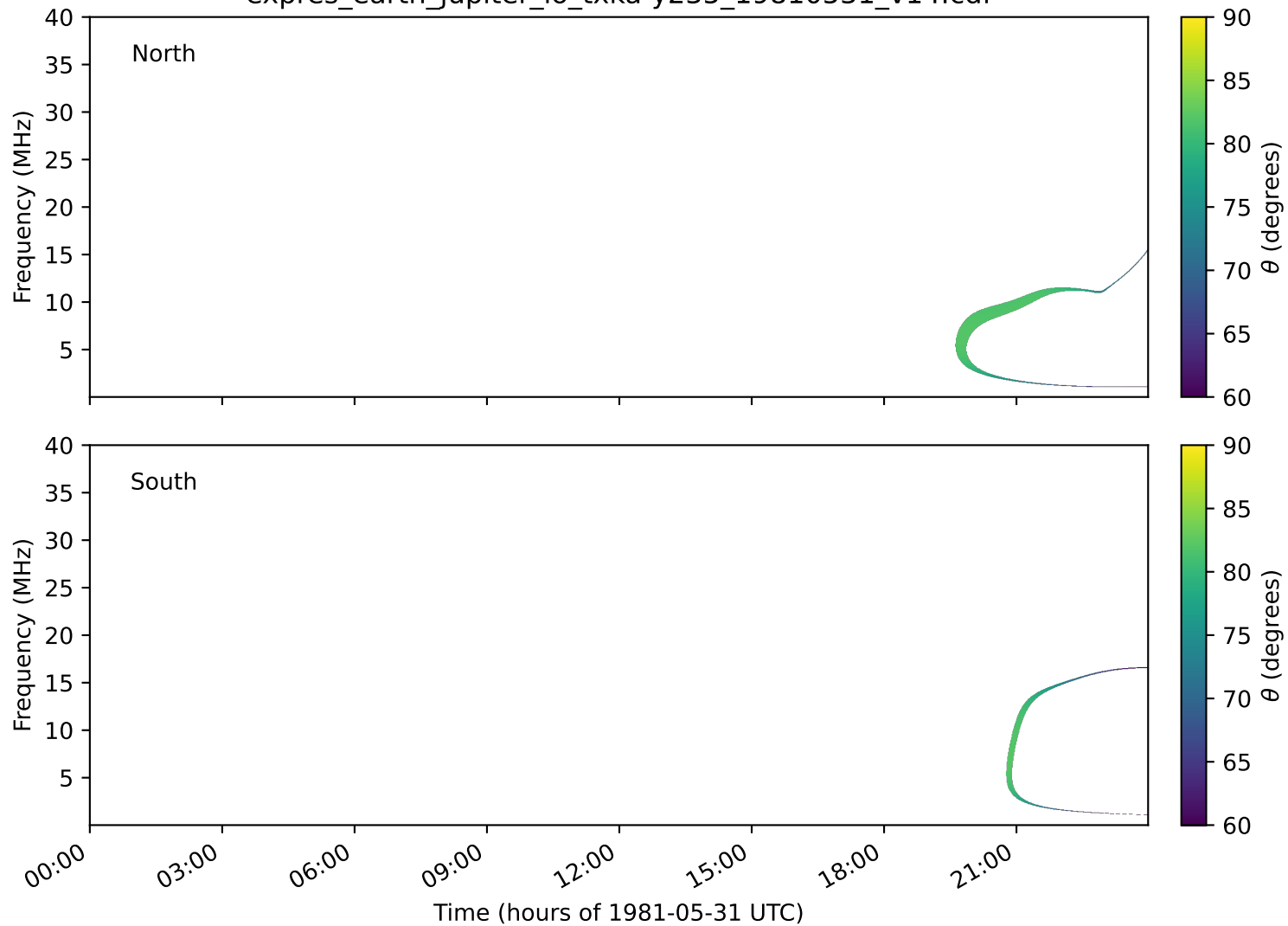
expres_earth_jupiter_io_txka-y235_19810531_v14.cdf
