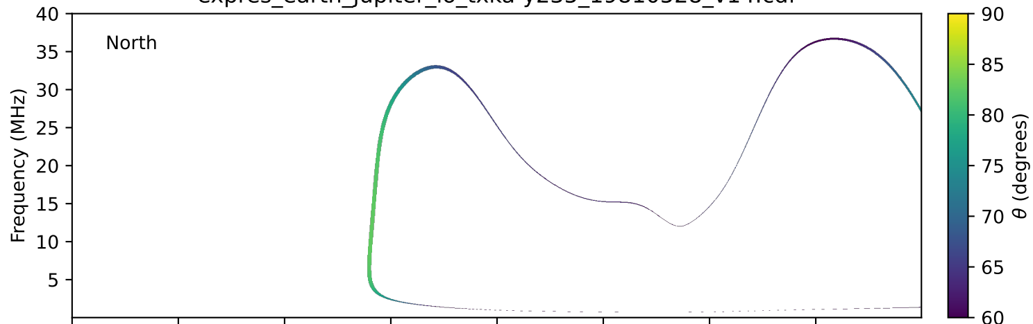
expres_earth_jupiter_io_txka-y235_19810528_v14.cdf
