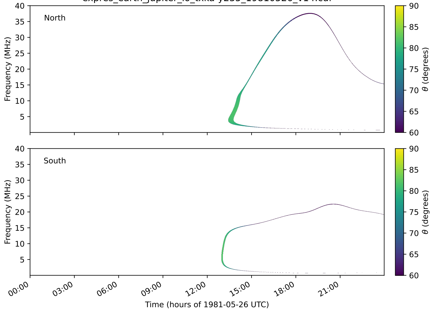
expres_earth_jupiter_io_txka-y235_19810526_v14.cdf
