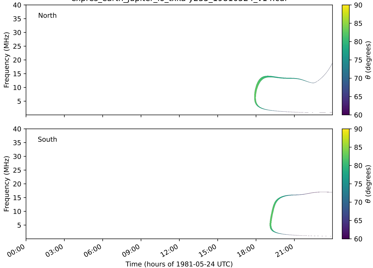
expres_earth_jupiter_io_txka-y235_19810524_v14.cdf
