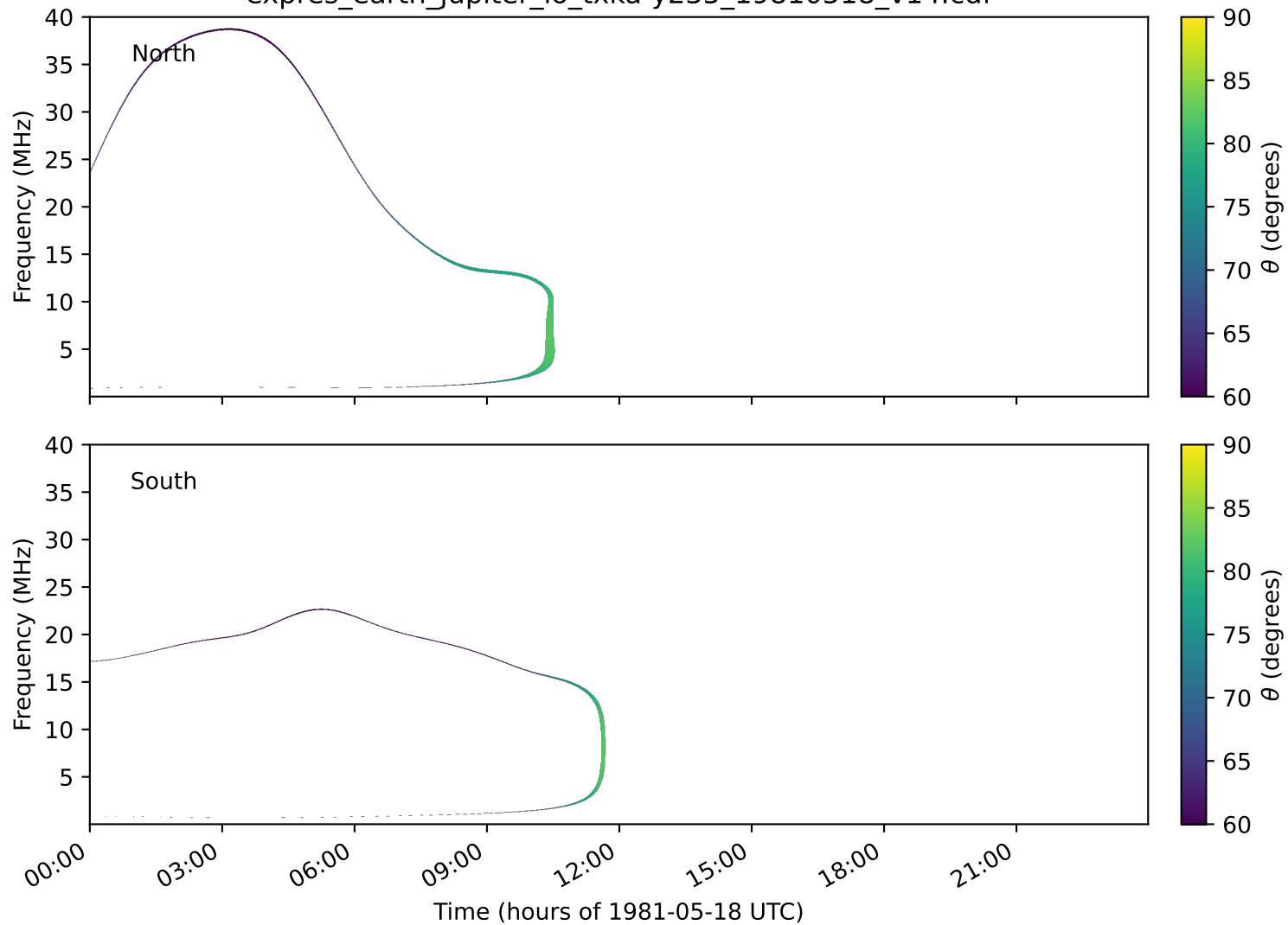
expres_earth_jupiter_io_txka-y235_19810518_v14.cdf
