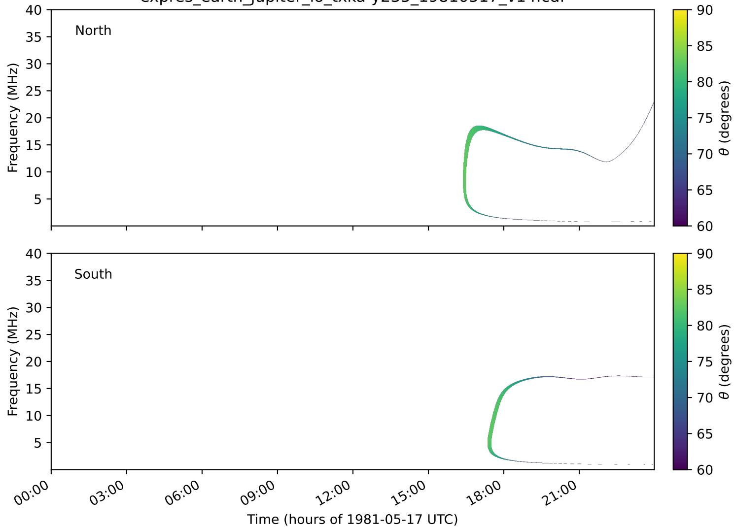
expres_earth_jupiter_io_txka-y235_19810517_v14.cdf
