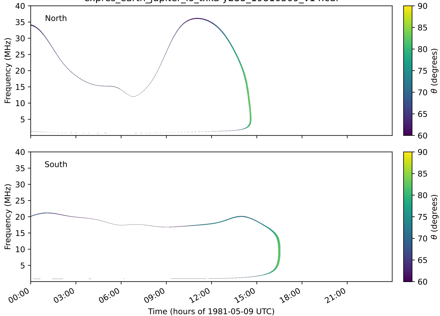
expres_earth_jupiter_io_txka-y235_19810509_v14.cdf
