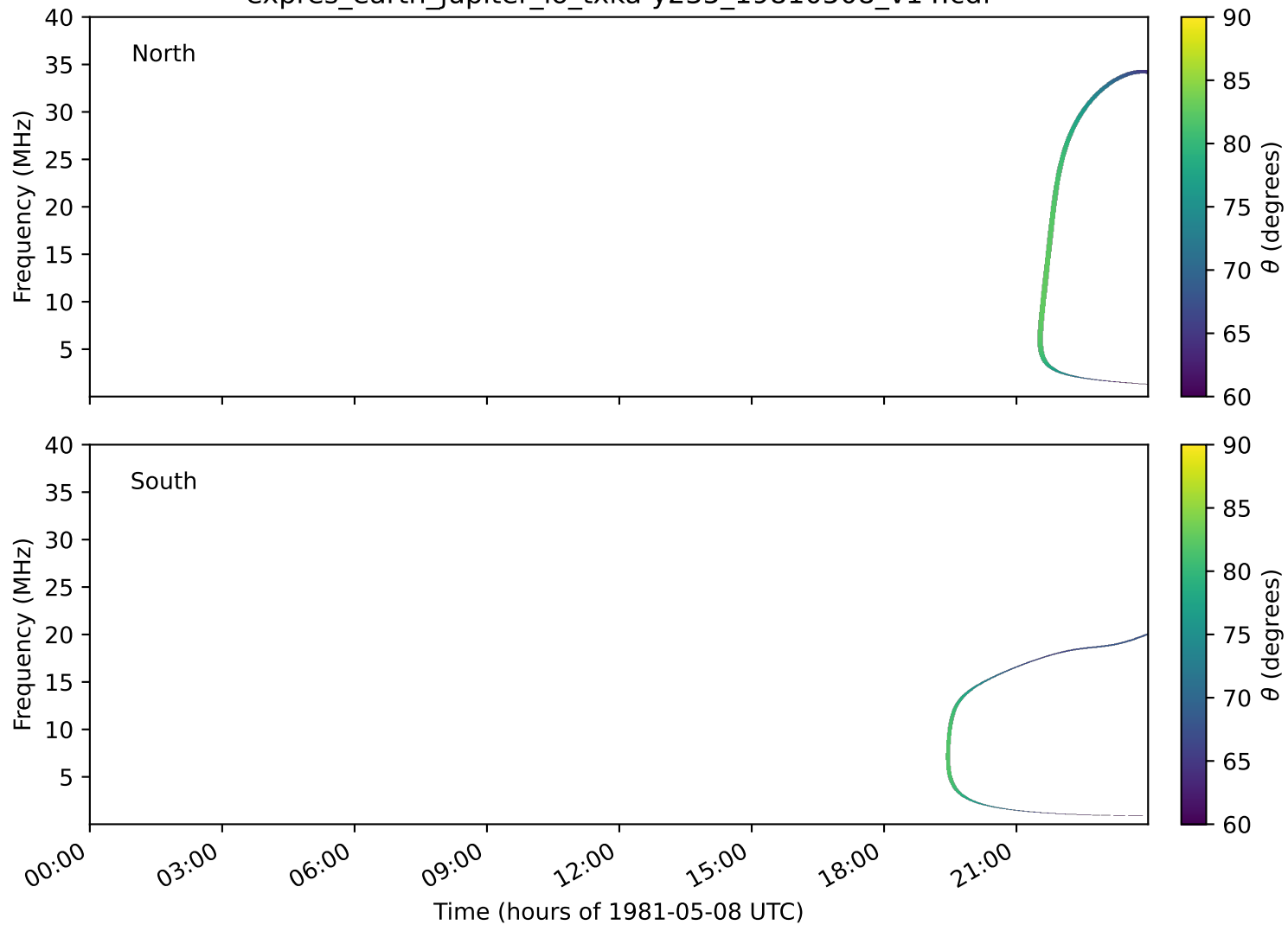
expres_earth_jupiter_io_txka-y235_19810508_v14.cdf
