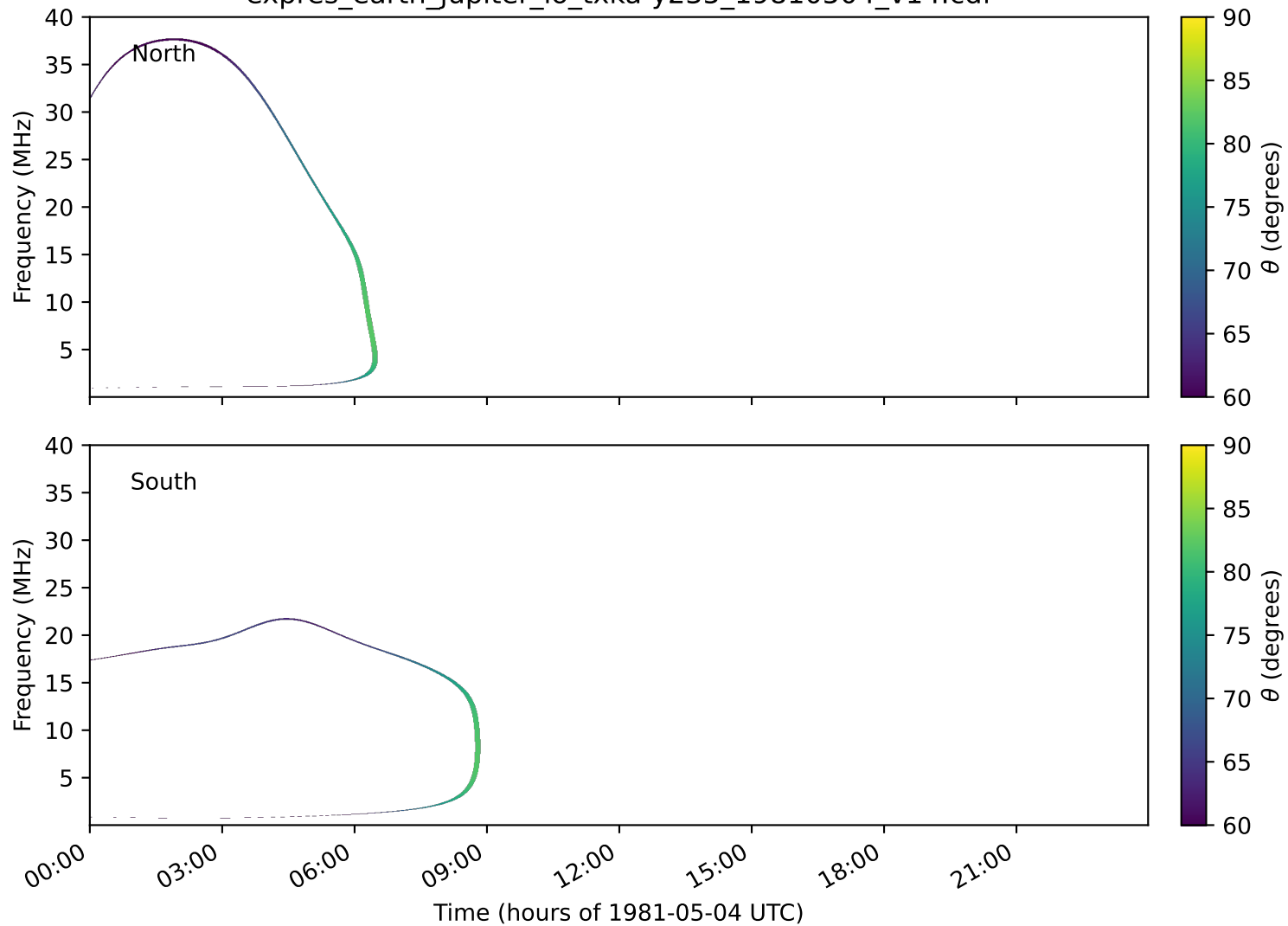
expres_earth_jupiter_io_txka-y235_19810504_v14.cdf
