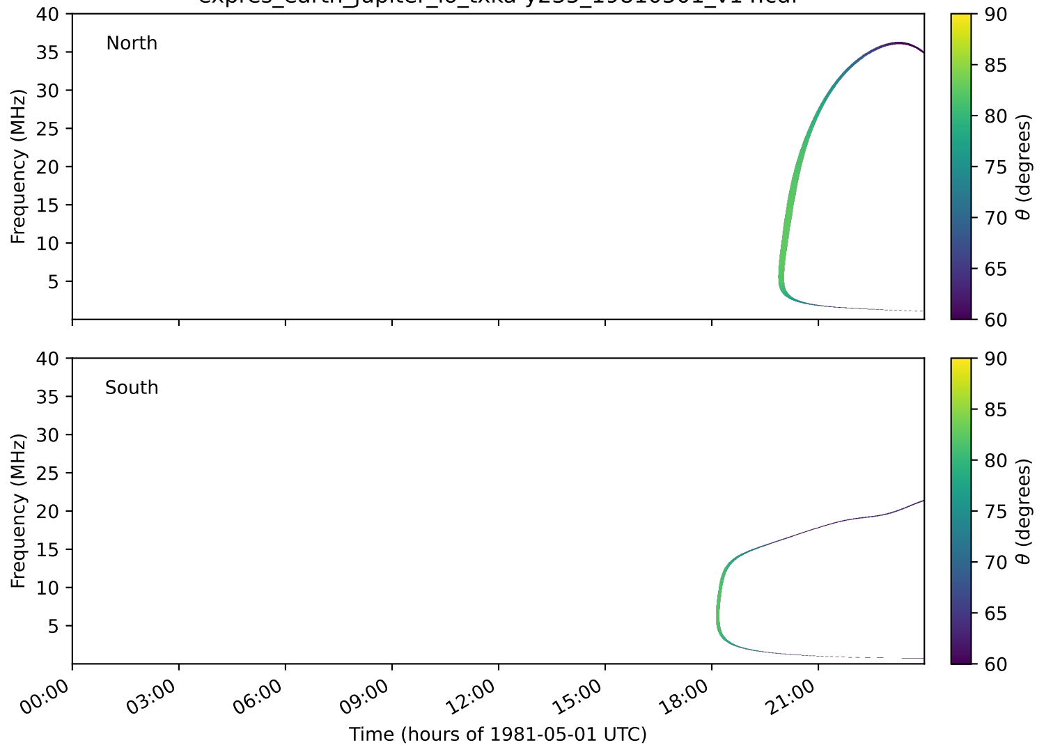
expres_earth_jupiter_io_txka-y235_19810501_v14.cdf
