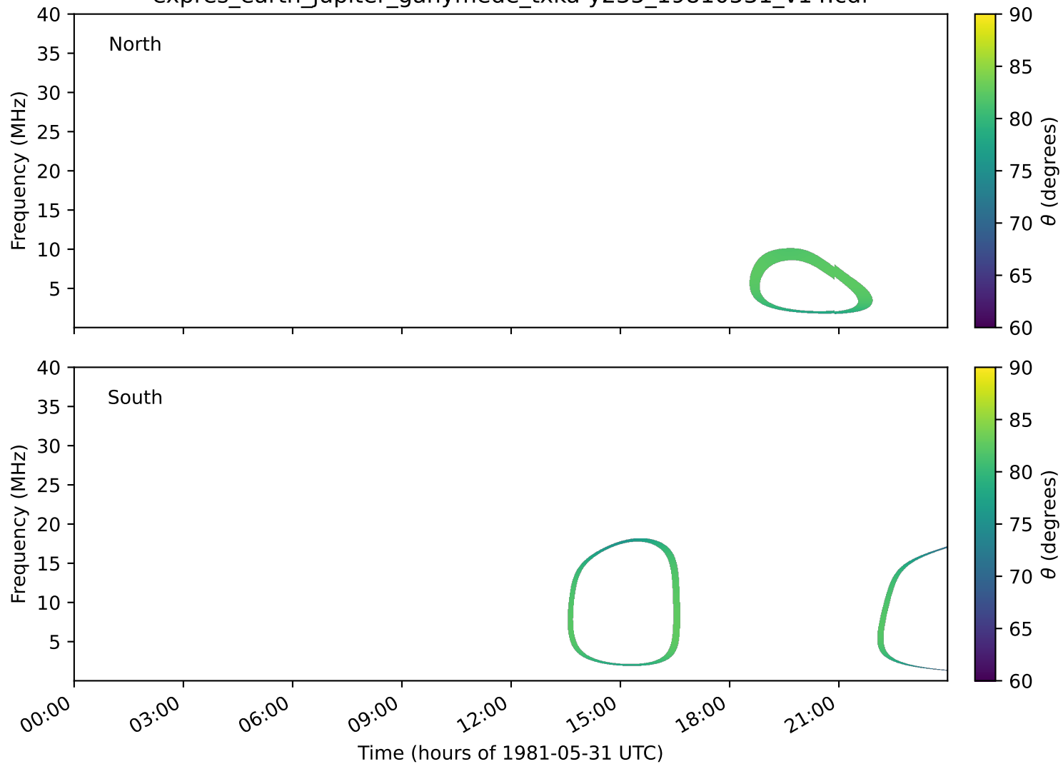
expres_earth_jupiter_ganymede_txka-y235_19810531_v14.cdf
