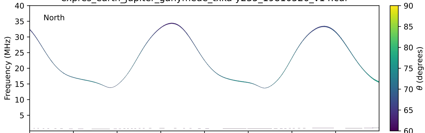
expres_earth_jupiter_ganymede_txka-y235_19810526_v14.cdf
