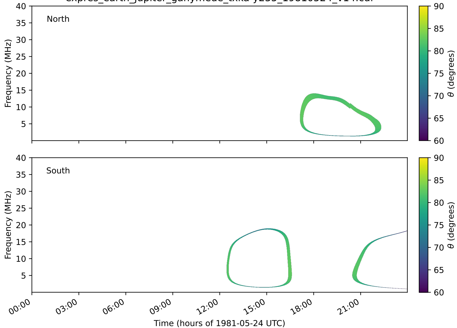
expres_earth_jupiter_ganymede_txka-y235_19810524_v14.cdf
