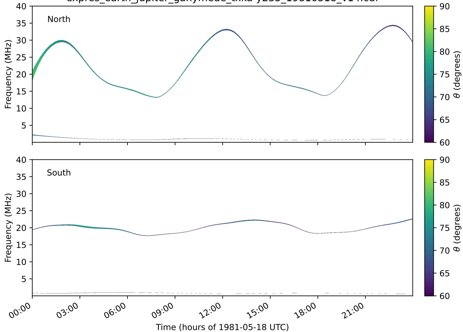
expres_earth_jupiter_ganymede_txka-y235_19810518_v14.cdf
