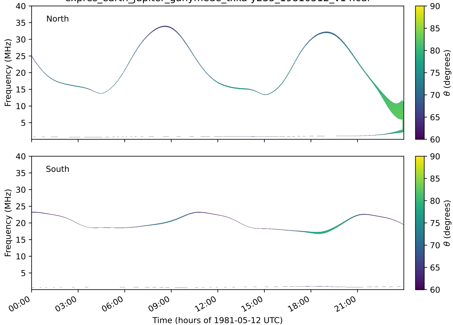
expres_earth_jupiter_ganymede_txka-y235_19810512_v14.cdf
