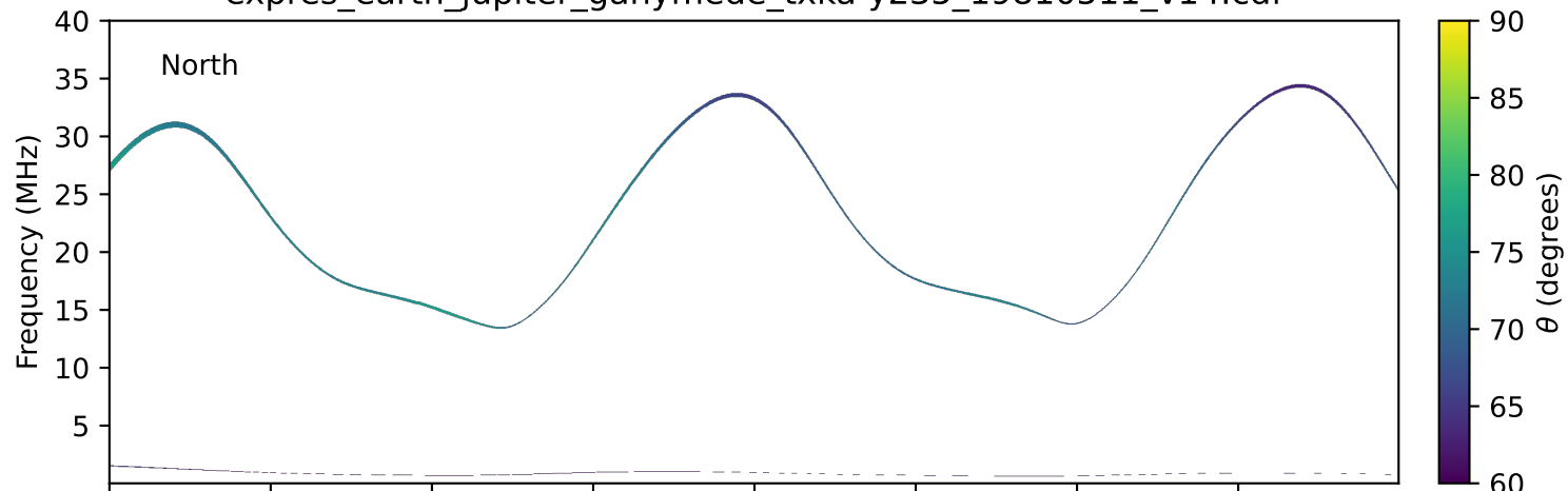
expres_earth_jupiter_ganymede_txka-y235_19810511_v14.cdf
