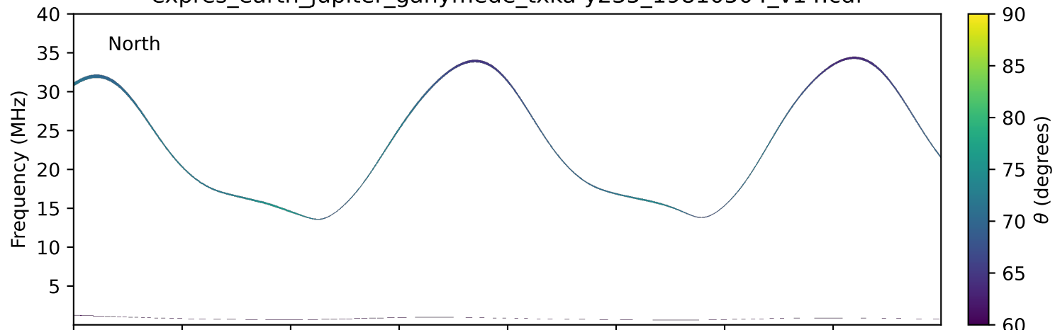
expres_earth_jupiter_ganymede_txka-y235_19810504_v14.cdf
