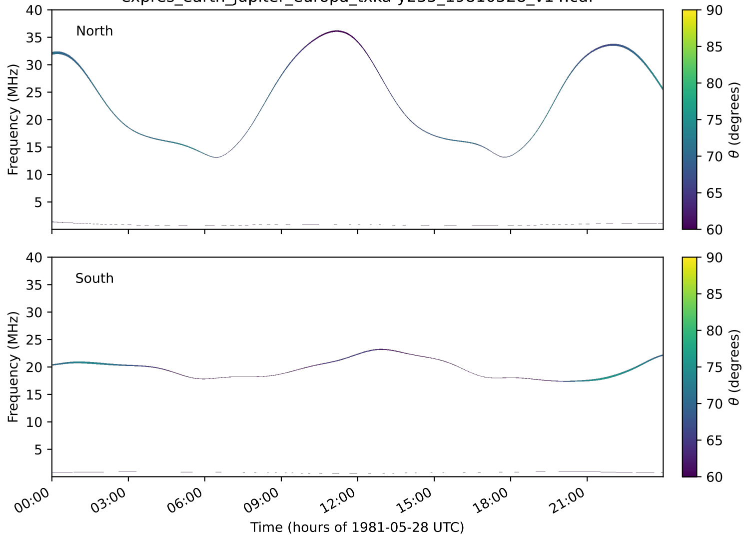
expres_earth_jupiter_europa_txka-y235_19810528_v14.cdf
