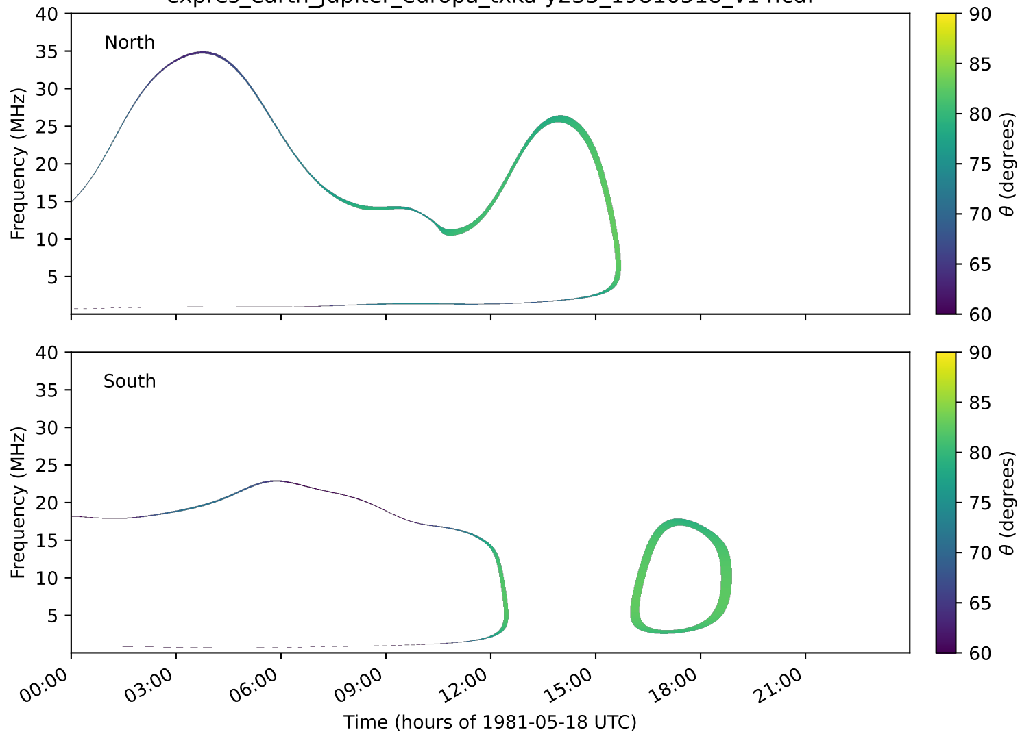
expres_earth_jupiter_europa_txka-y235_19810518_v14.cdf
