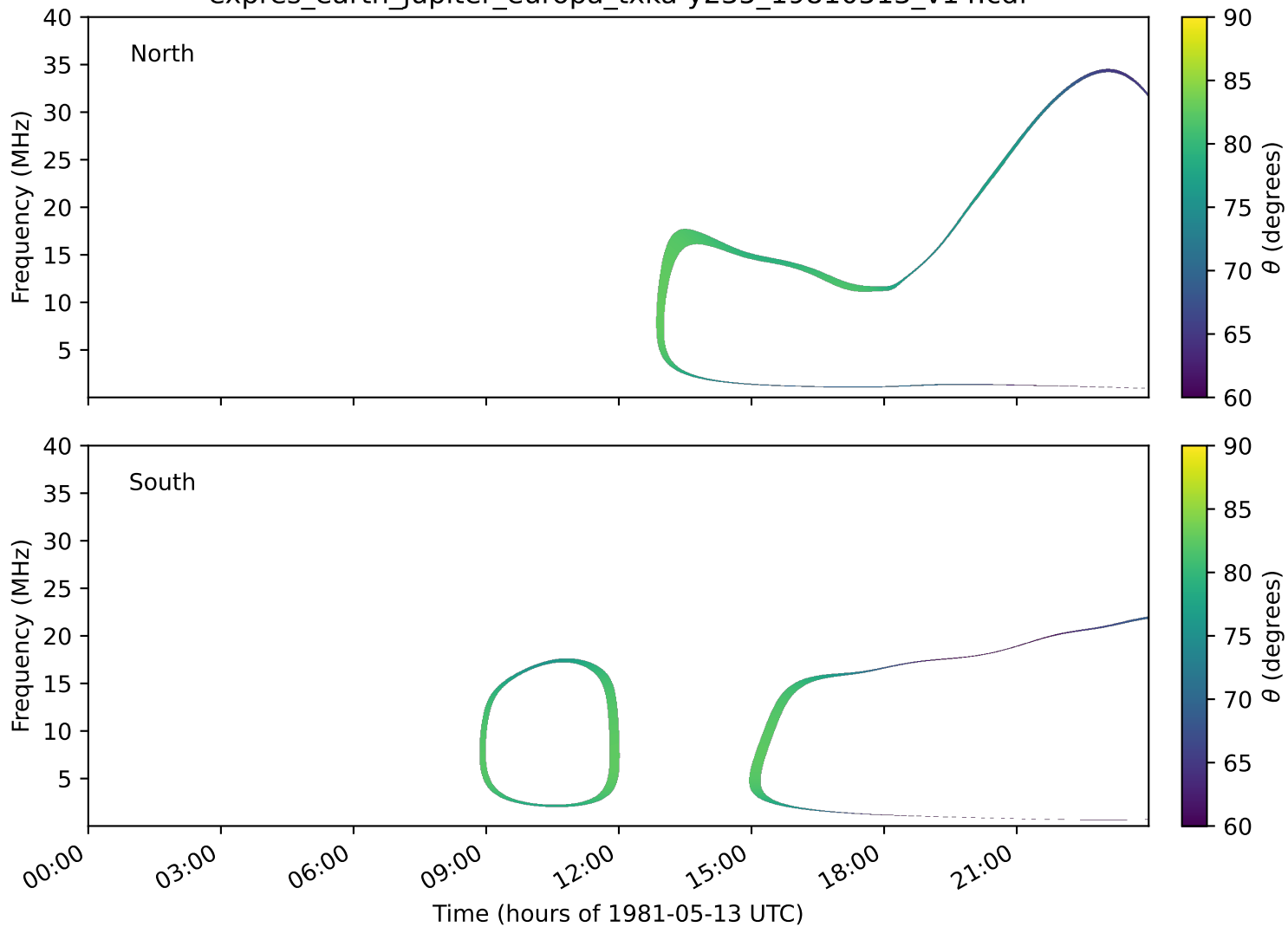
expres_earth_jupiter_europa_txka-y235_19810513_v14.cdf
