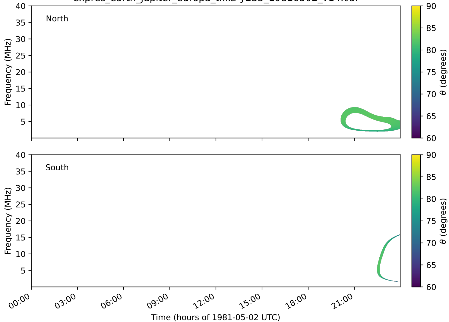
expres_earth_jupiter_europa_txka-y235_19810502_v14.cdf
