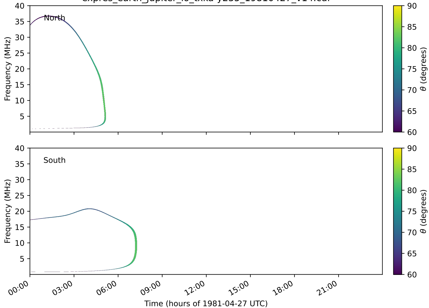
expres_earth_jupiter_io_txka-y235_19810427_v14.cdf
